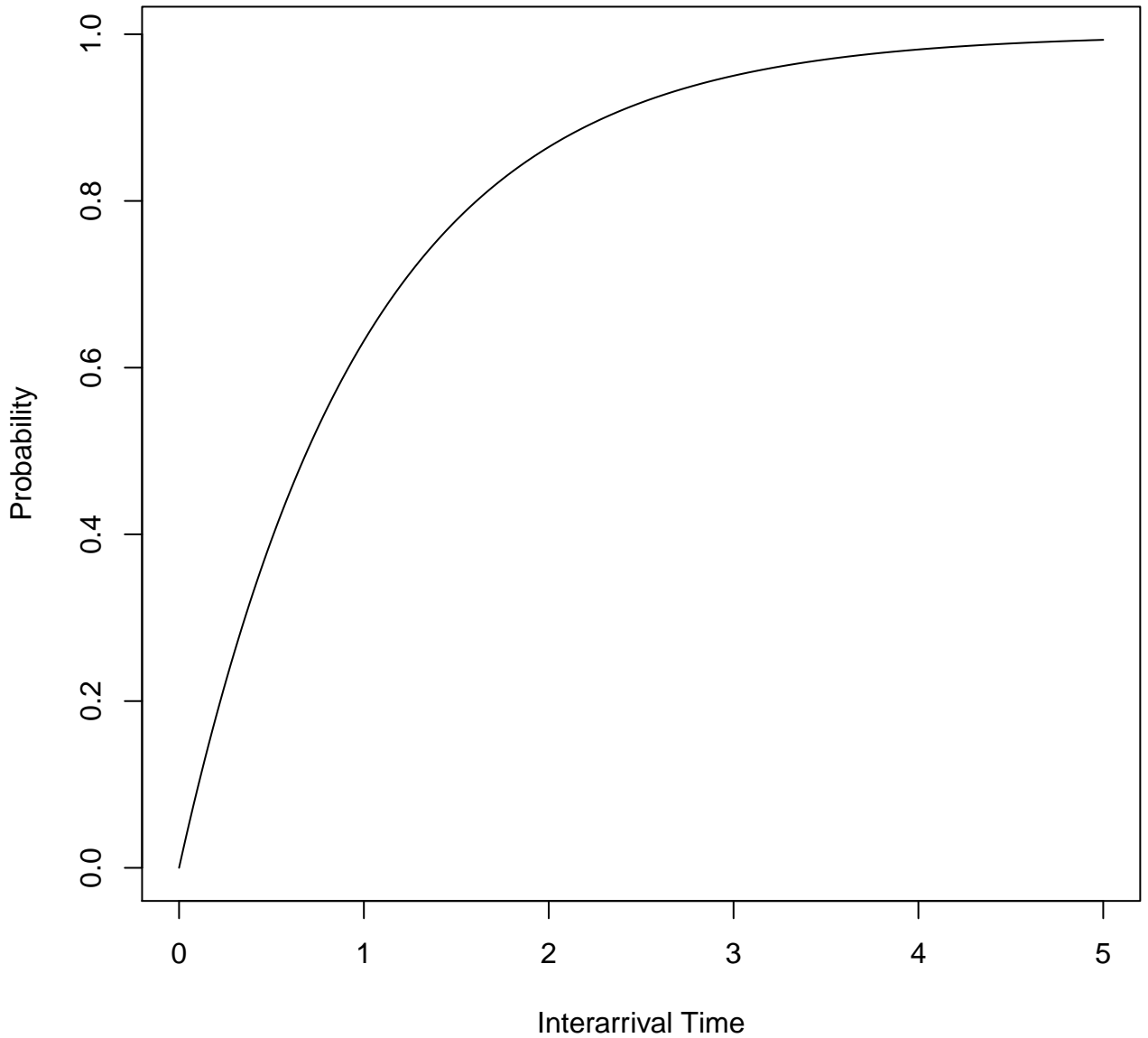
CDF of Exponential Distribution, lambda=1
