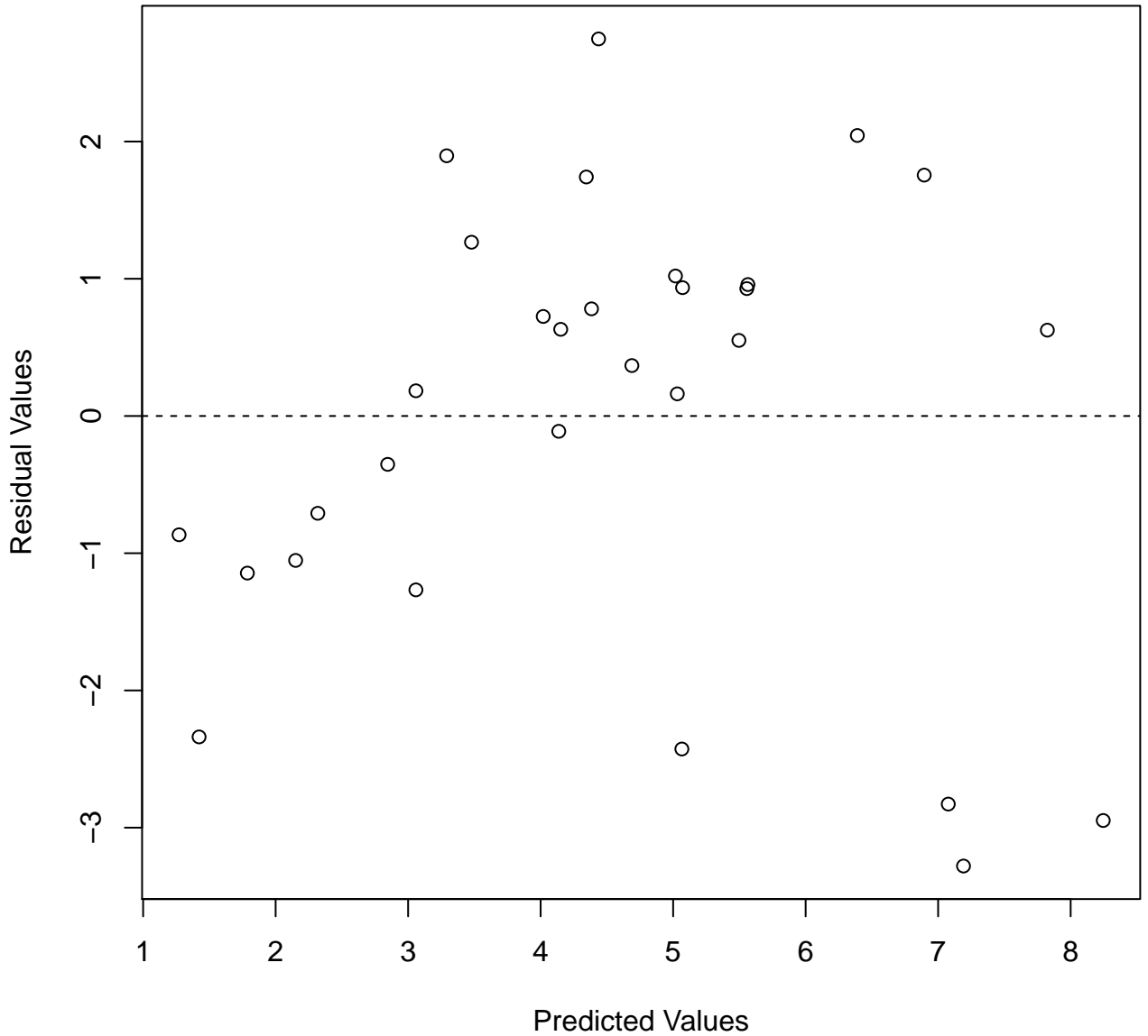
Model 2: Residual Plot
