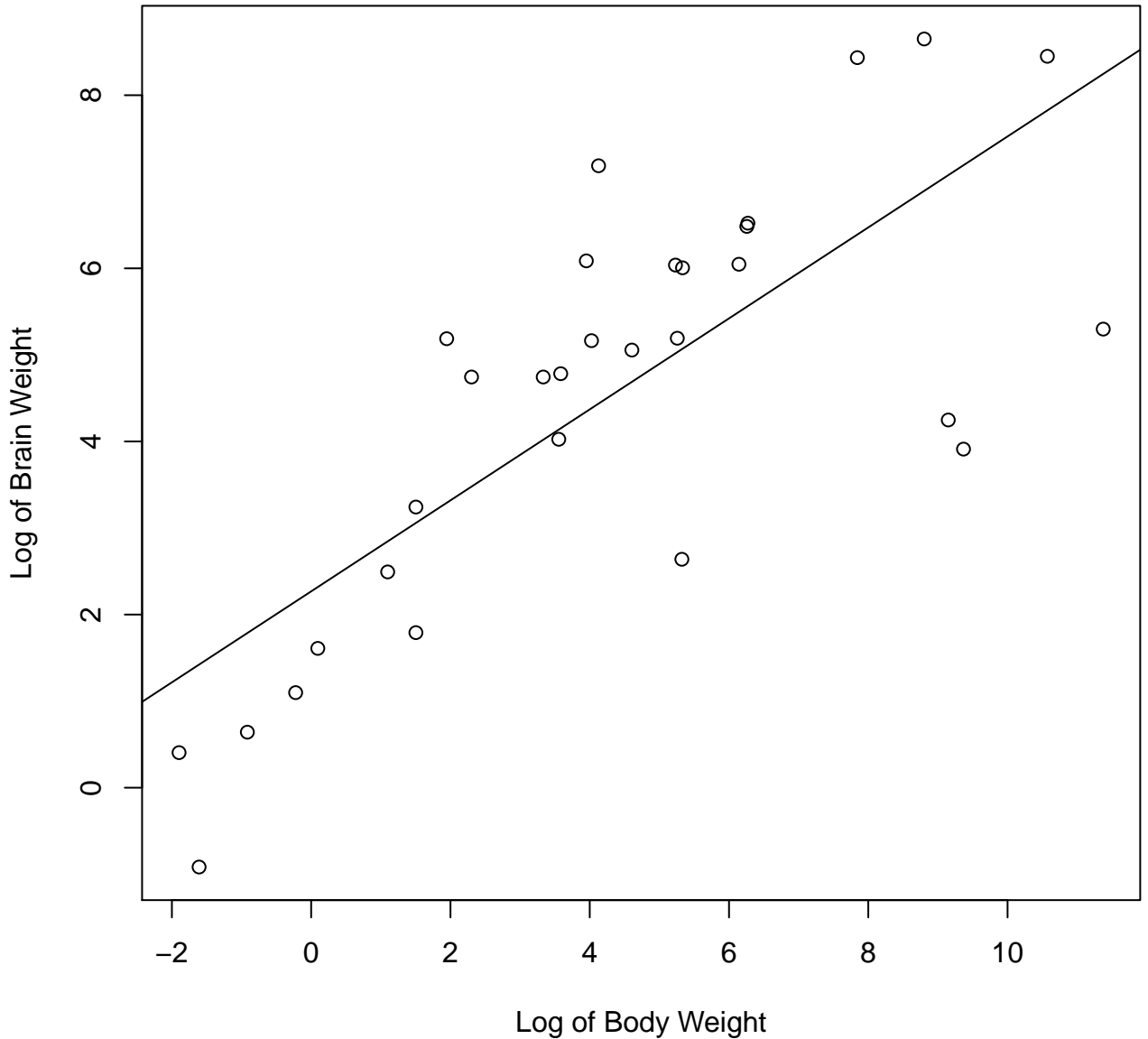
Scatterplot of Log(BrainWeight) vs. Log(BodyWeight)
