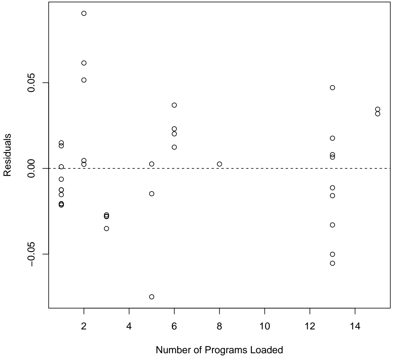
Residual Plot 3
