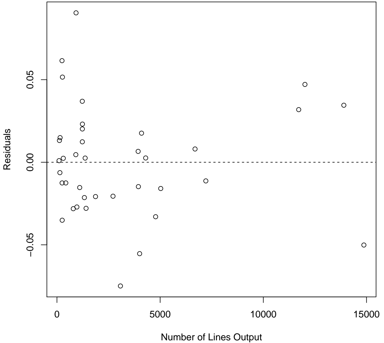
Residual Plot 2
