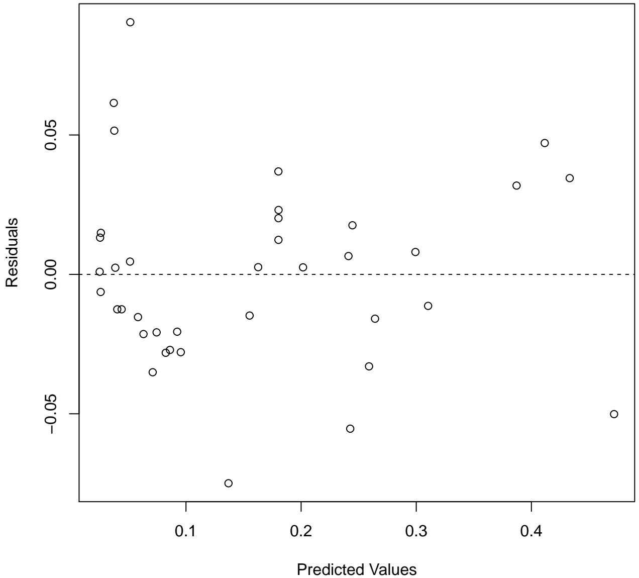
Residual Plot 1
