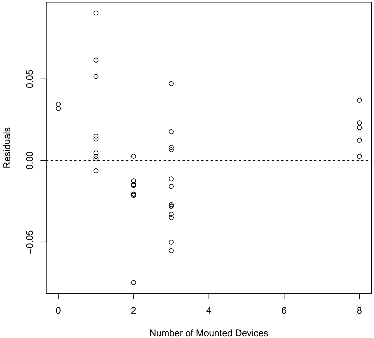
Residual Plot 4
