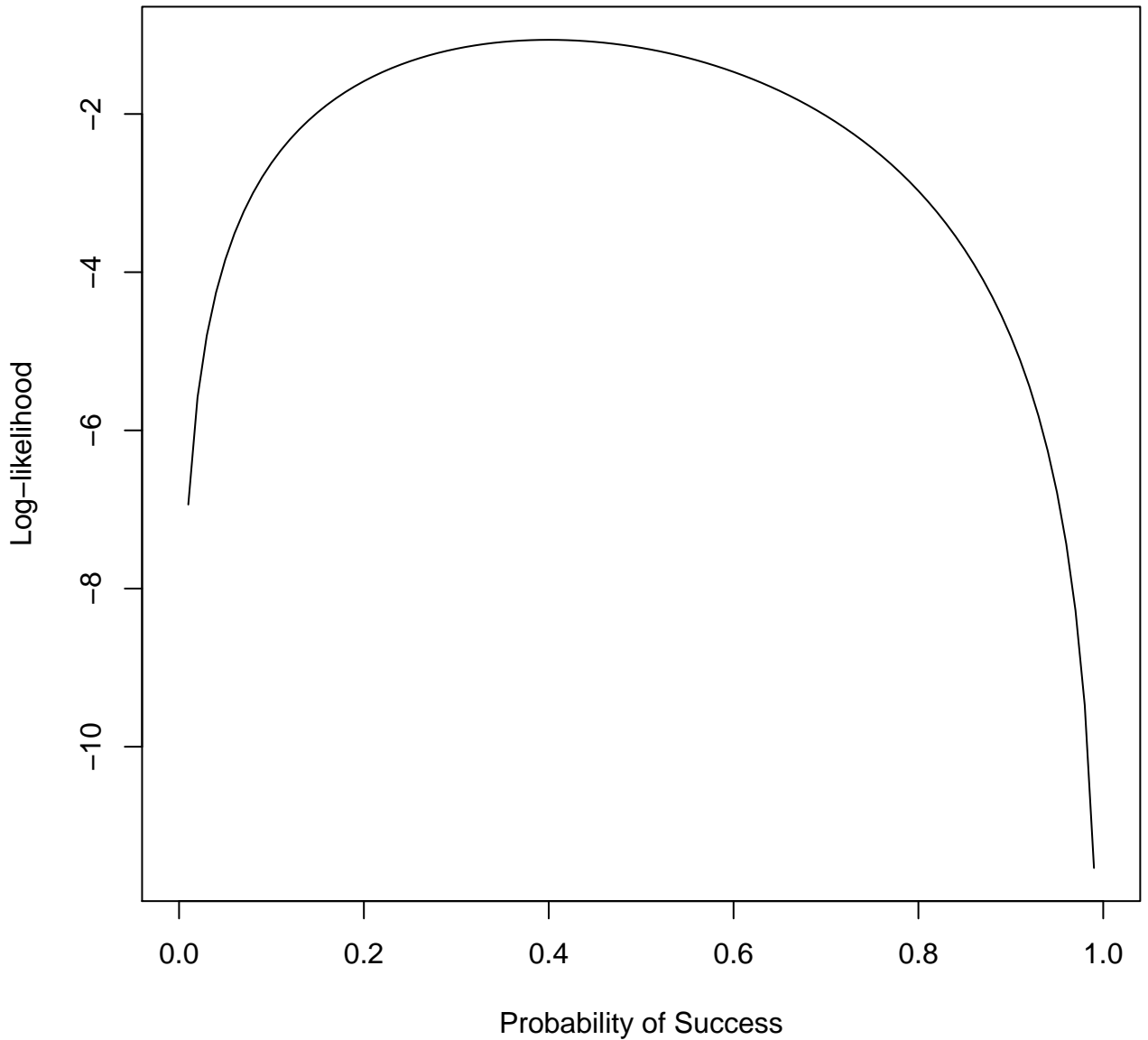
Plot of log-likelihood for Bernoulli Distribution
